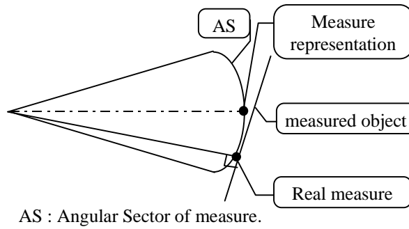
Figure 9: Measure representation.
