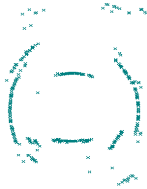
Figure 1: Ultrasonic measures in a room without obstacle.
