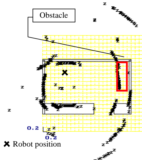
Figure 15: Set of points with only first echoes.
