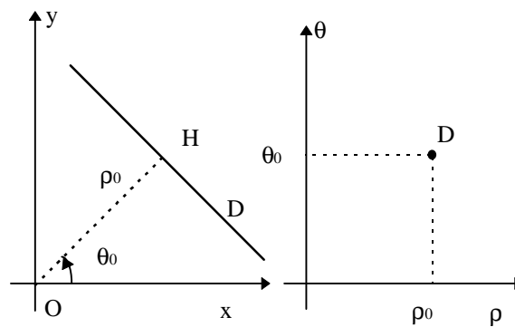
Figure 4: Hough transform representation.
