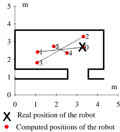
Figure 12: Localisation example without obstacle.
