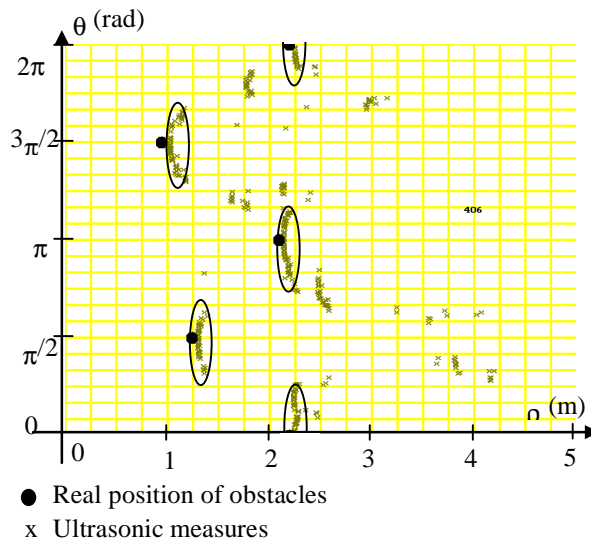
Figure 10: Uncertainty ellipsis of a straight line in a plane.
